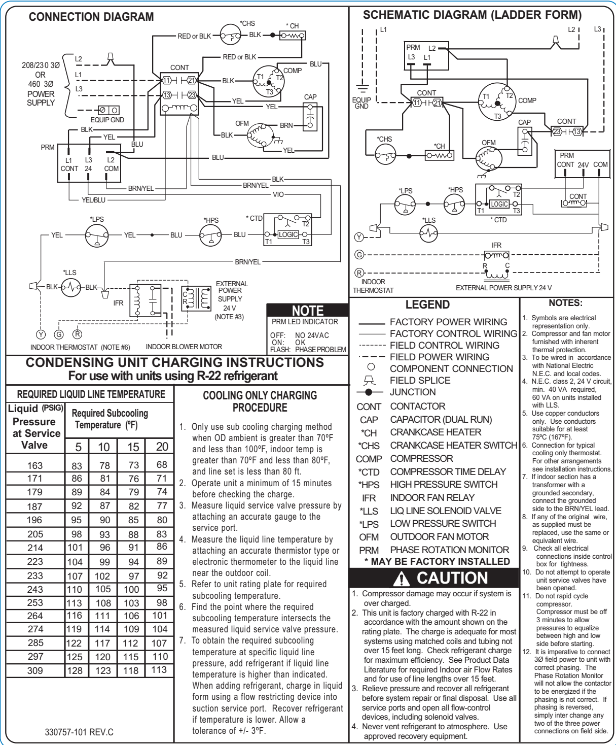
Fig. 2 – Wiring Diagram — Model sizes 2-1/2 - 5 tons, 208/230-3 and Model sizes 3 - 5 tons, 460-3
